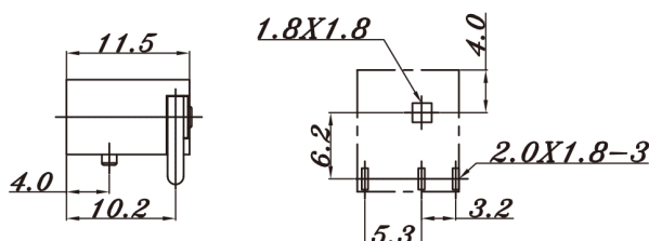
P.C.B LAYOUT BOTTOM VIEW
