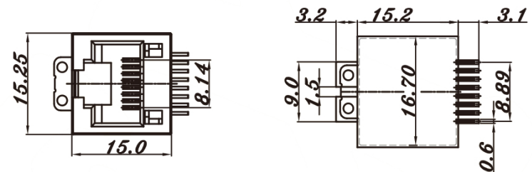
PCB LAYOUT/TOP VIEW
