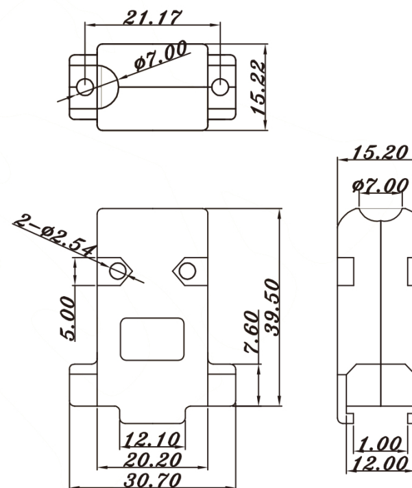
45D Exit 9 Pin
