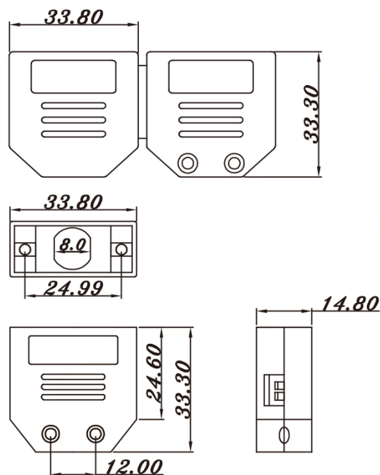
Folding Type 15 Pin
