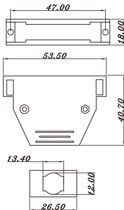
Buckle Type 25 Pin
