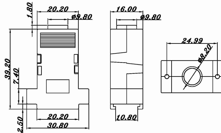
Snap-In Type 9 Pin
