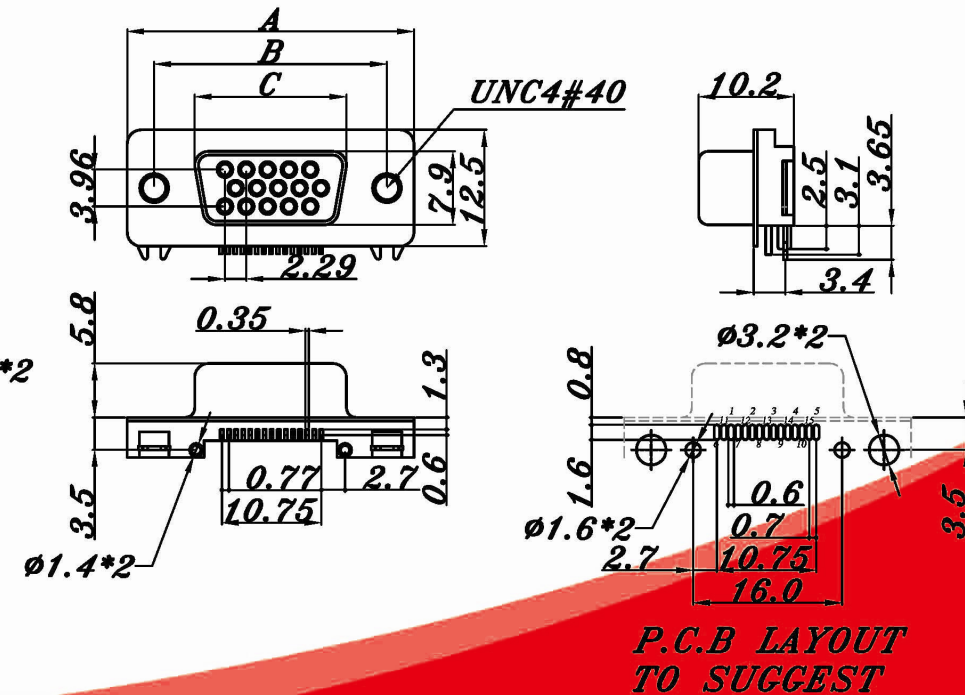
427B DIP
