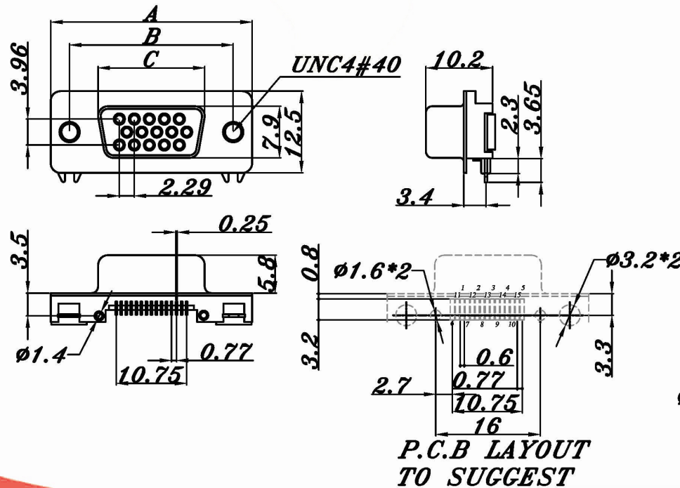
427A SMD
